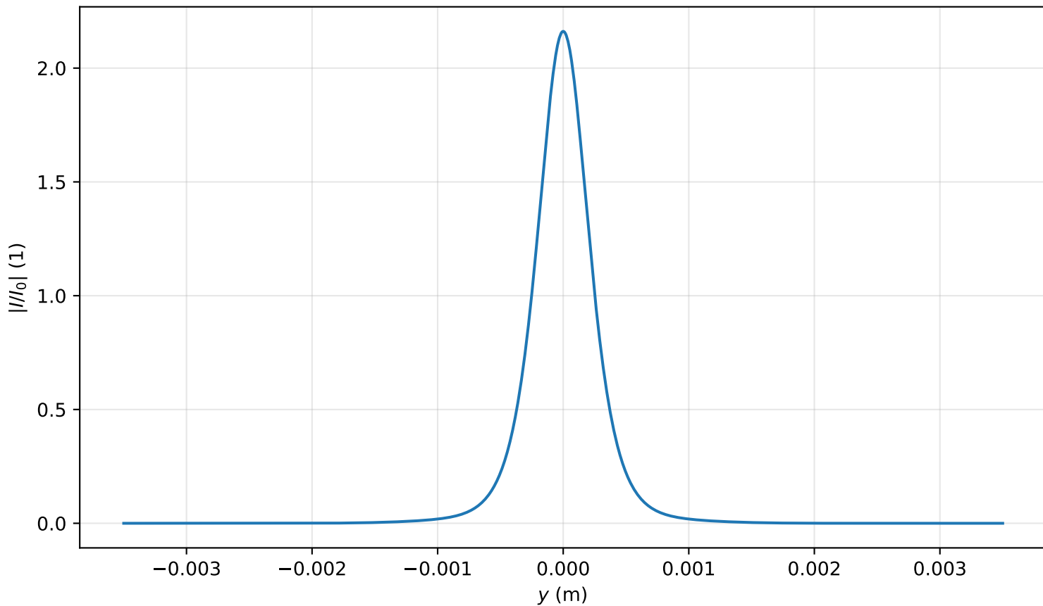
Intensity profile I(x=0, y, z=2.070)/I_0 , \text{Pin}=1.0\text{Pcr} , artificial time
